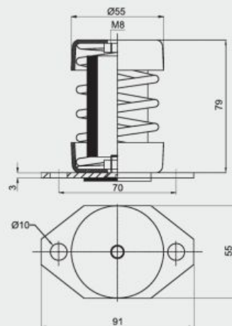
Dimensions AM-25 to AM-125
