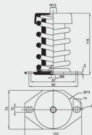
Dimensions AM-250
